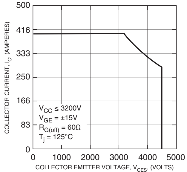
REVERSE BIAS SAFE OPERATING AREA (RBSOA)
