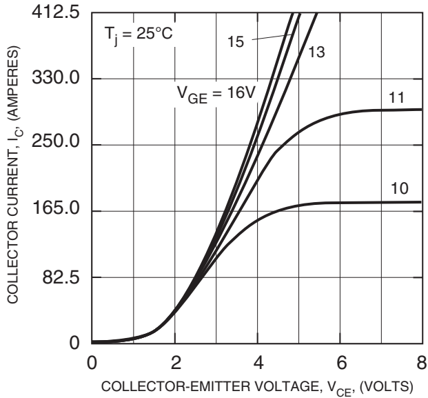
OUTPUT CHARACTERISTICS (TYPICAL)
