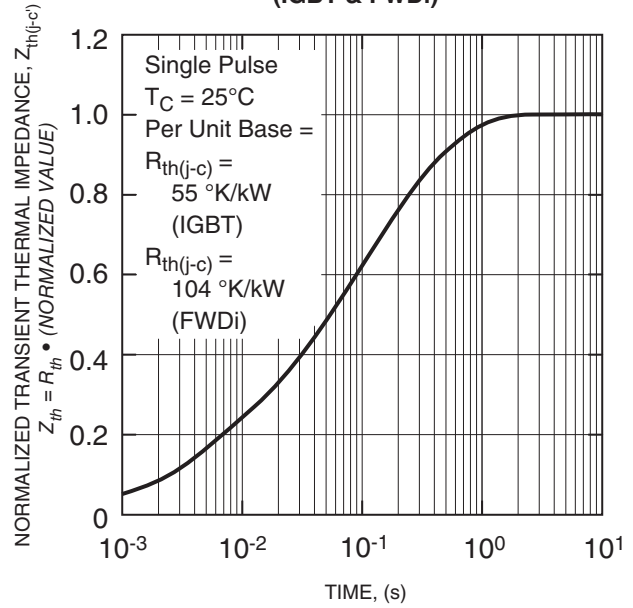
TRANSIENT THERMAL IMPEDANCE CHARACTERISTICS (IGBT & FWDi)
